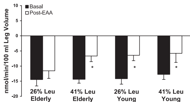
Fig. 7. Average responses for the leg phenylalanine net balance ( \text{nmol}\cdot\text{min}^{-1}\cdot 100\text{ ml leg volume}^{-1} ) for the basal state (Basal) and after the ingestion of 6.7 g of EAAs (Post-EAA) containing either 1.7 (26% Leu) or 2.8 (41% Leu) g of leucine. *Significantly different from the corresponding basal value ( P < 0.05 ).
