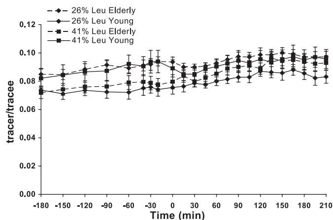
Fig. 3. Mean arterial blood L-[ring- 2 H 5 ]phenylalanine enrichment of phenylalanine (tracer-to-tracee ratio) in the basal state and after the ingestion of 6.7 g of EAAs containing either 1.7 (26% Leu) or 2.8 (41% Leu) g of leucine at 0 min.
